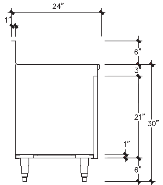
SECTION (CUSTOM)
