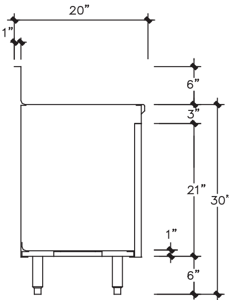
SECTION (PRO-LINE)
