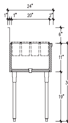
SECTION (NCIB)
