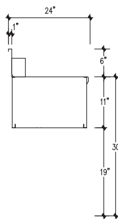
SECTION (NCWD-BC)
