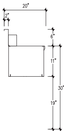
SECTION (NPWD-BC)
