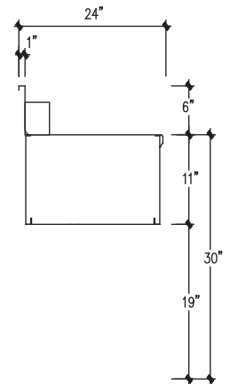
SECTION (NCWD-BW)
