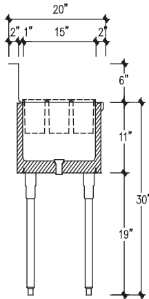
SECTION (NPIB)
