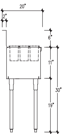
SECTION (NPWD-BW)
