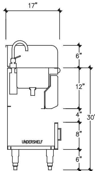
SECTION (CABINET)
