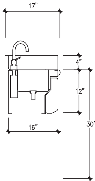
SECTION (DROP-IN)
