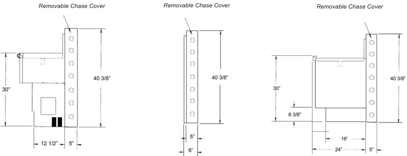
Pedestal Module End View
